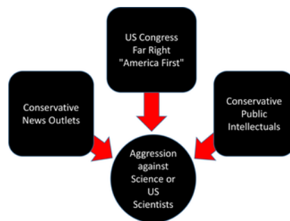
Fig 1. Aggression against science or US scientists in the Year 2021.
